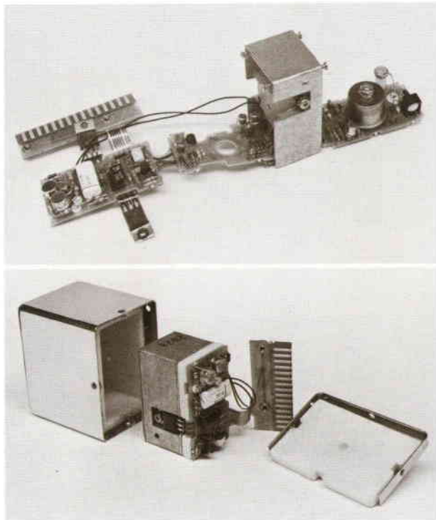
Fig. 3. Final assembly of 10811A/B Oscillator.
