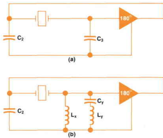
Fig. 7. The SC-cut crystal in the 10811A/B Oscillator is mode-suppressed to allow only C-mode operation. This diagram shows a standard Colpitts-type oscillator (top) and the same oscillator with mode suppression.
