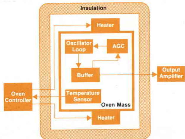
Fig. 6. Block diagram of the 10811A/B Oscillator. The oscillator loop includes a 10-MHz SC-cut quartz crystal.
