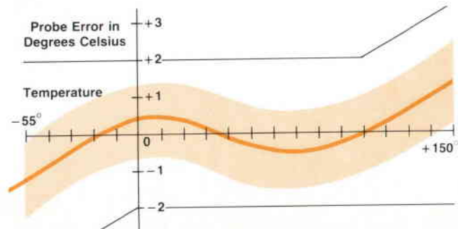
Fig. 4. Typical 10023A error curve with possible unit-to-unit variations (shaded band).
