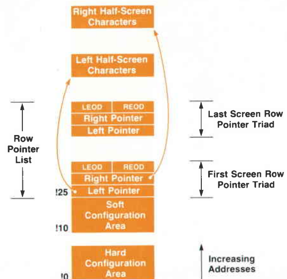
Fig. 2. The display memory contains two configuration areas, a pointer list, and the rows of characters to be displayed.
