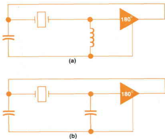
Fig. 8. Equivalent circuits for the mode-suppression circuit of Fig. 7. Top: low and high-frequency equivalent circuit. Bottom: passband equivalent circuit.
